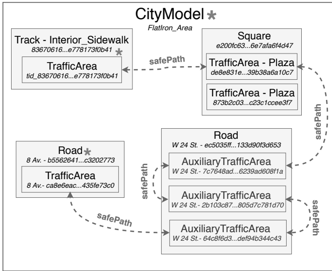
(b) Fragment of the corresponding view generated.
